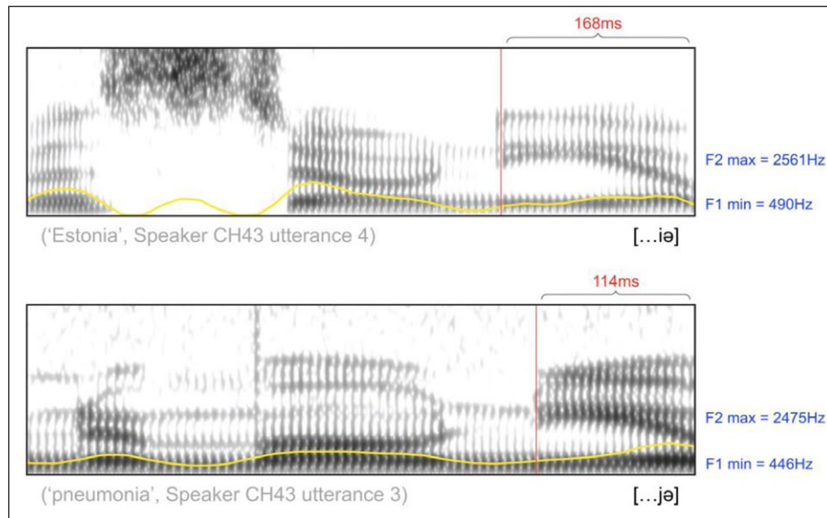
Figure 1: Example utterance spectrograms. Spectrograms of utterances by the same speaker of a near-minimal pair expecting and appearing to exhibit the distinction of interest. The vertical red line shows the vocalic onset and the end of the spectrogram is where the vocalic offset was segmented, with the duration of the entire vocalic sequence noted. The yellow line is Praat's intensity tracker. The F2 max and F2 min of each vocalic sequence of interest are also noted.
