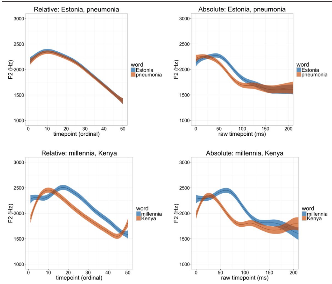
Figure 4: Smoothing Spline ANOVA plots. Plots on the lefthand side represent the x-axis in Relative terms, with 50 timepoints (evenly spaced across the entire vocalic sequence duration) expressed ordinally. Plots on the righthand side are in Absolute terms, with the x-axis converted to the amount of time (ms) between each point and the onset of the vocalic sequence. In each plot, the earlier half is that containing the high front vocoid of primary interest; the latter half represents the following vowel and also some indication of the transition into the initial segment of the following word.
