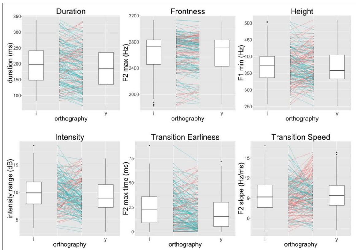
Figure 3: Nonce stimuli. Visualizations provide box plots across the two orthography conditions. Points represent the measurement for each speaker's utterance of each nonce stimulus (averaged across repetitions and grouped by orthography alongside the respective box plot). Lines connect each pair's counterparts, with a green line representing that [i] > [j] and a red line representing that [i] < [j].
