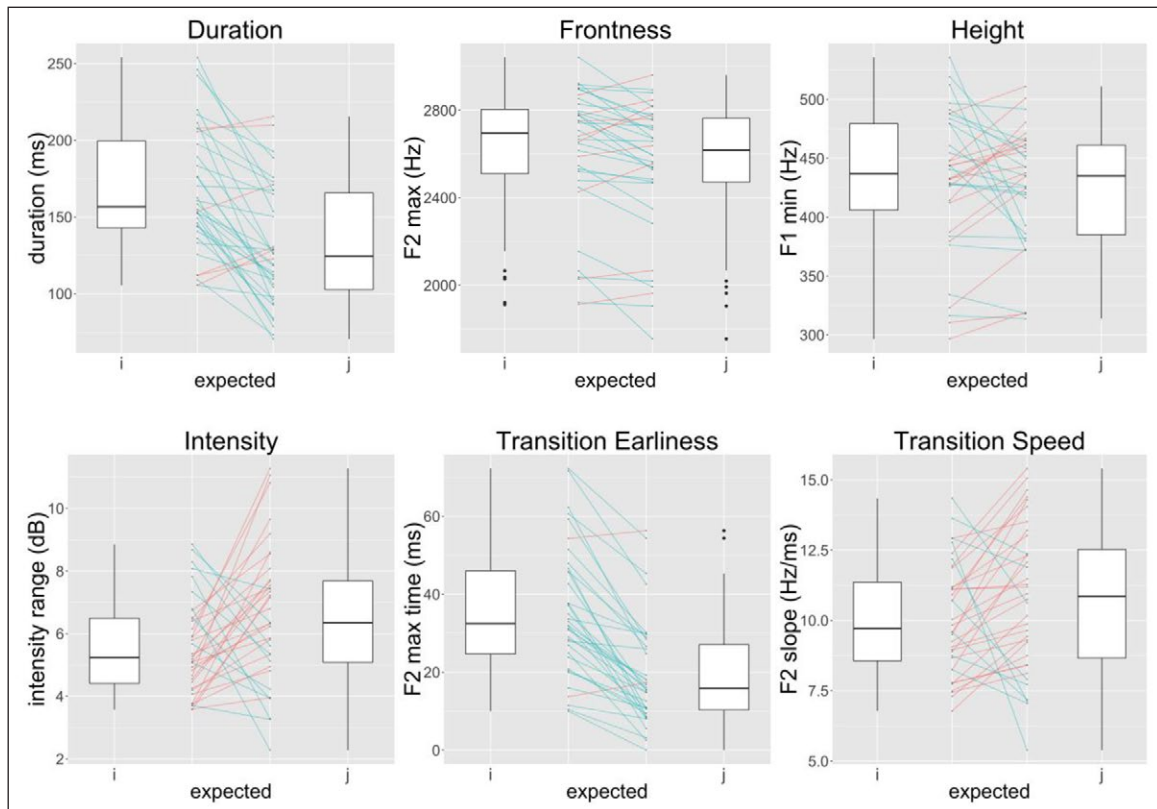
Figure 2: Pre-existing lexical items. Visualizations provide box plots across the two expected pronunciation conditions. Points represent the measurement for each speaker's utterance of each word (averaged across repetitions and grouped by expected pronunciation alongside the respective box plot). Lines connect each pair's counterparts, with a green line representing that [i] > [j] and a red line representing that [i] < [j] .
